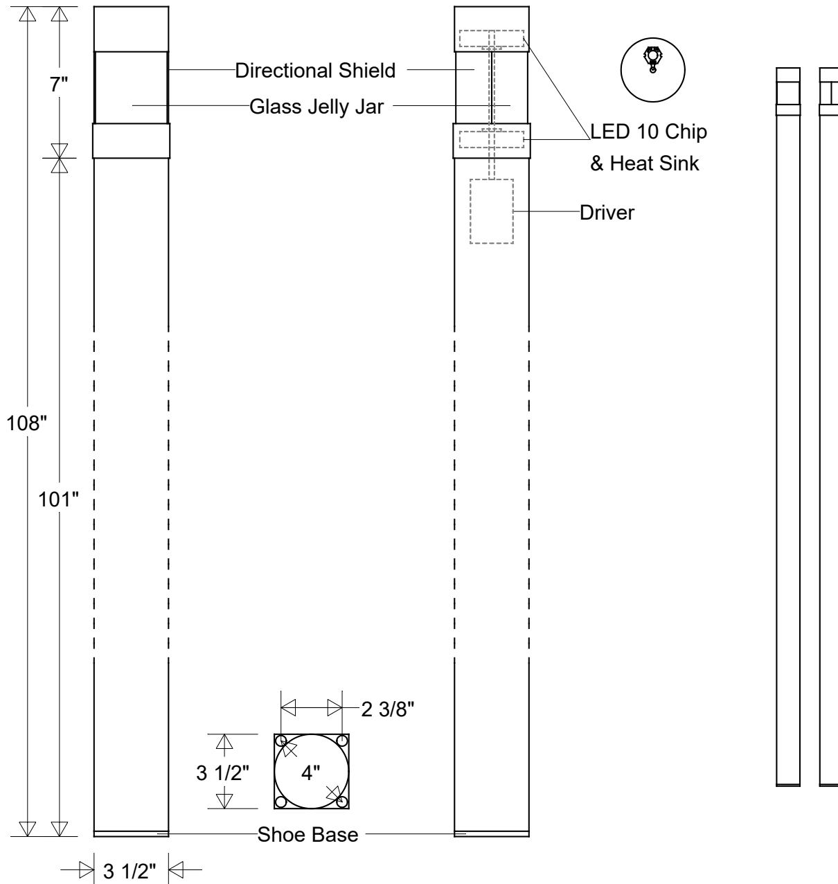
FRONT VIEW
