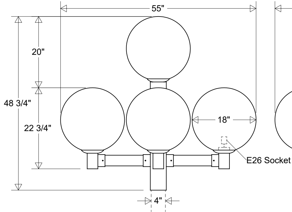
SIDE VIEW
