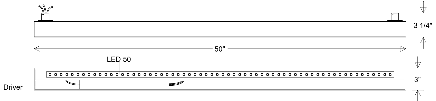
FRONT/INSIDE VIEW
