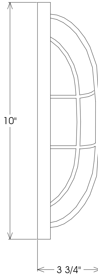
side view
