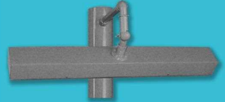
#5744/1855-13 ESW LED 25 12" OAH | 17 5/8" OAE | 24" OAL Light Box: 24" L | 2" H | 3" W Arm: 12" H | 13" Ext | 90° Swivel
